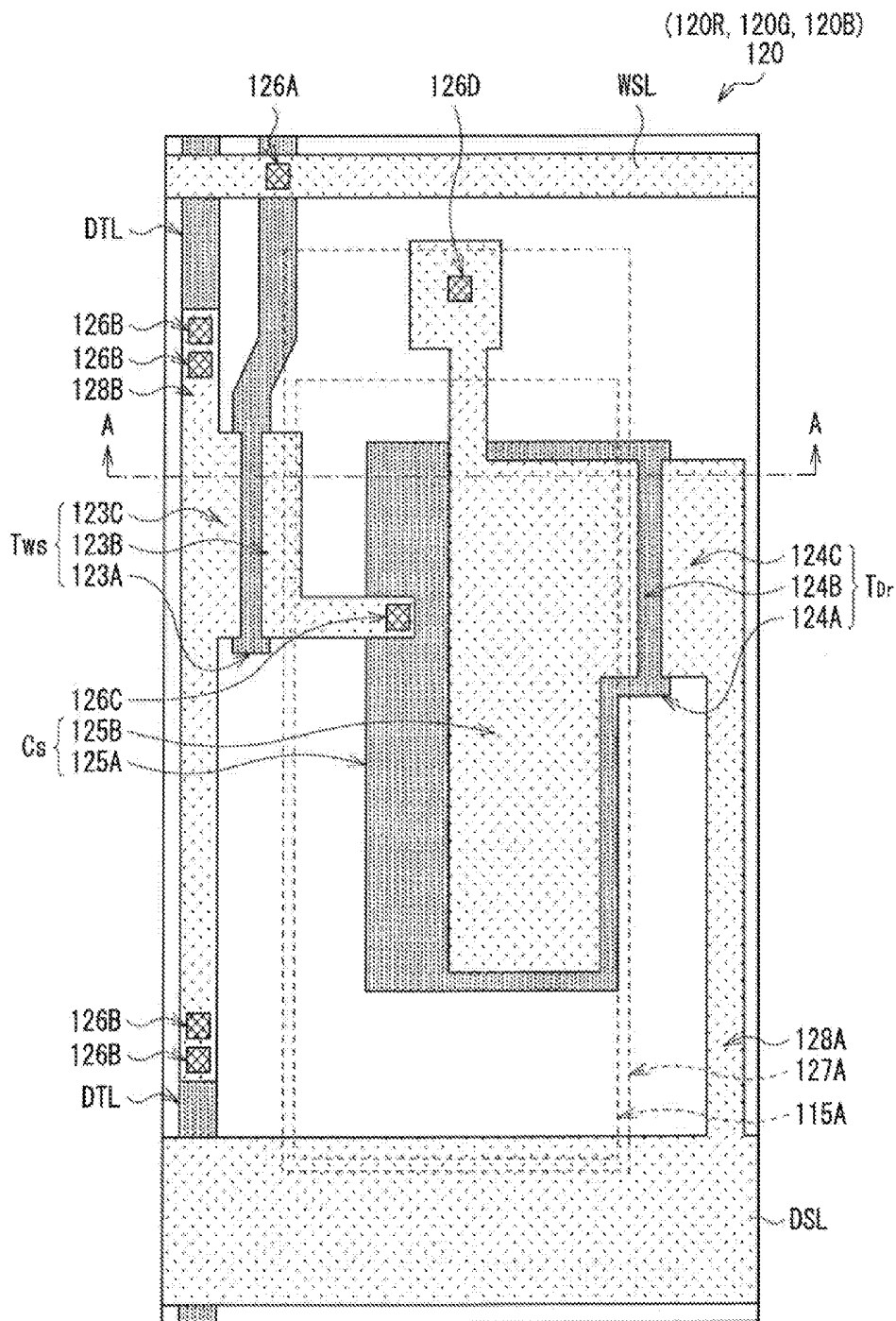
FIG. 17 PRIOR ART
